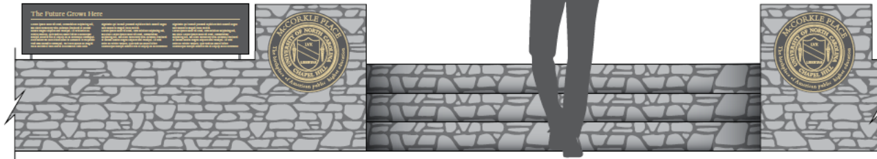
1 GATEWAY SIGN, NORTH ENTRANCE FRONT ELEVATION SCALE: 3/4"=1'-0"
